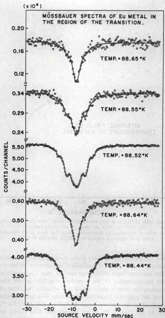
FIG. 3.— Spectra of Eu metal in the temperature region of the phase transition. The spectra are shown (from the top) in order of the time at which they were taken. The solid line is the result of a least-squares fit assuming that the absorption resulted partly from a "split" spectrum like those in Figure 1 and partly from a single line. This is equivalent to the assumption that paramagnetic Eu (unsplit spectrum) and ordered Eu (split) coexist over a narrow temperature range. Parameters evaluated from the least-squares fits are plotted in Figures 4 and 5.
