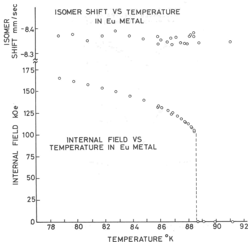
FIG. 2a. — Observed internal fields plotted as a function of temperature. Note the sudden drop of the field at T_1 . The (1\sigma) error flags are about the size of the points.
